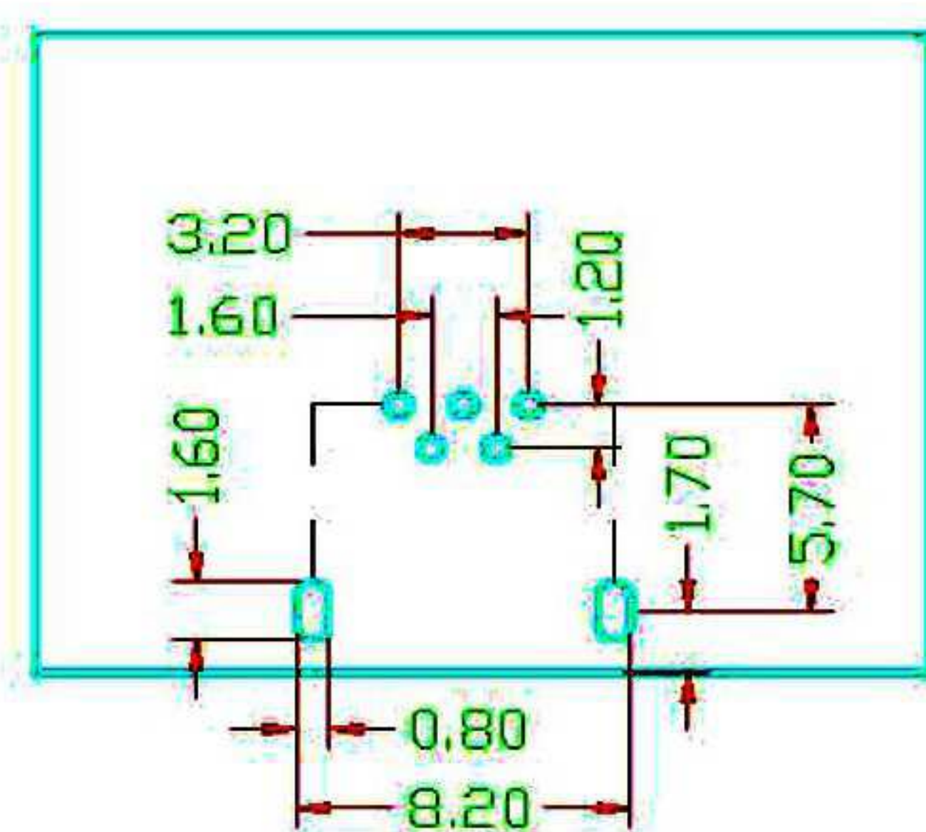
P.C.B. LAYOUT SCALE 2.00
