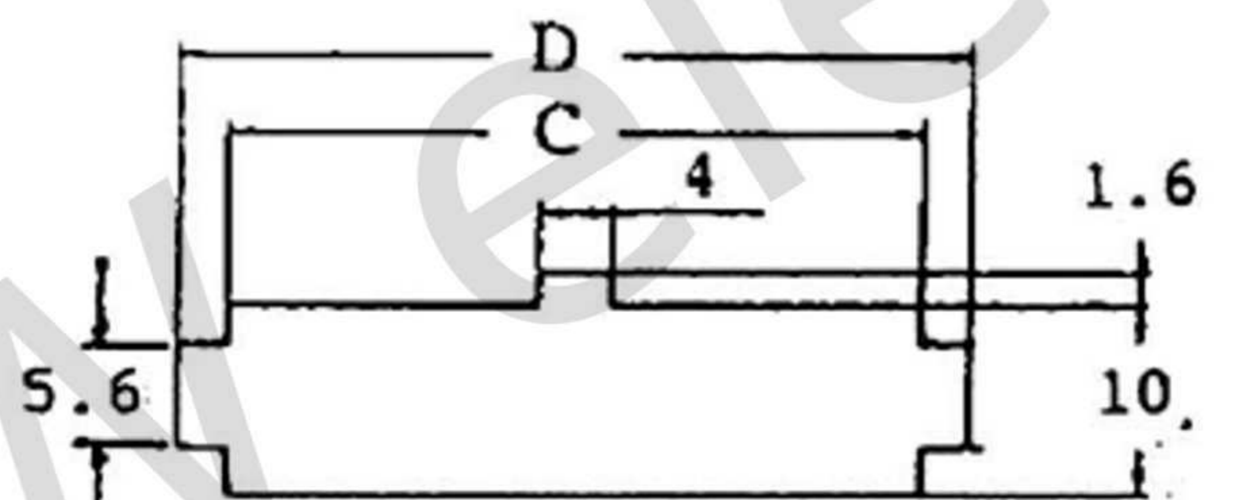
Mounting Hole Details for 259-NE Housing
