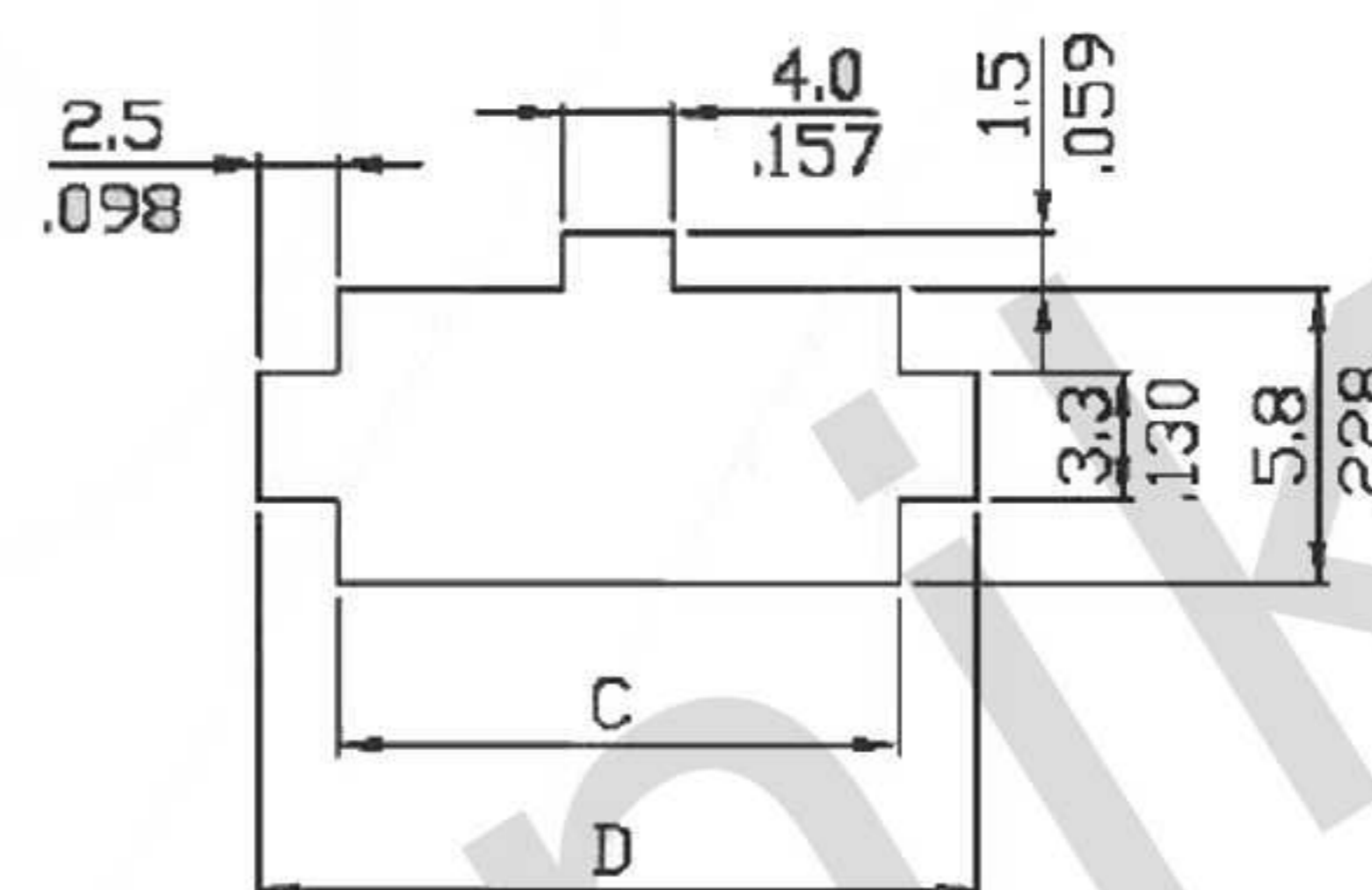
Panel Layout
